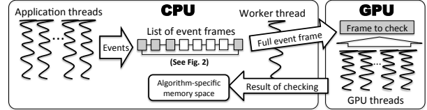
Figure 1. Components of our runtime monitoring system.
